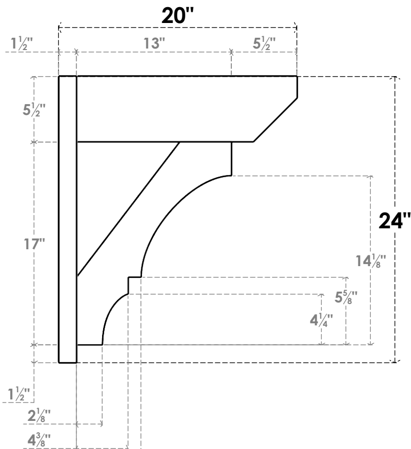
SIDE PROFILE
